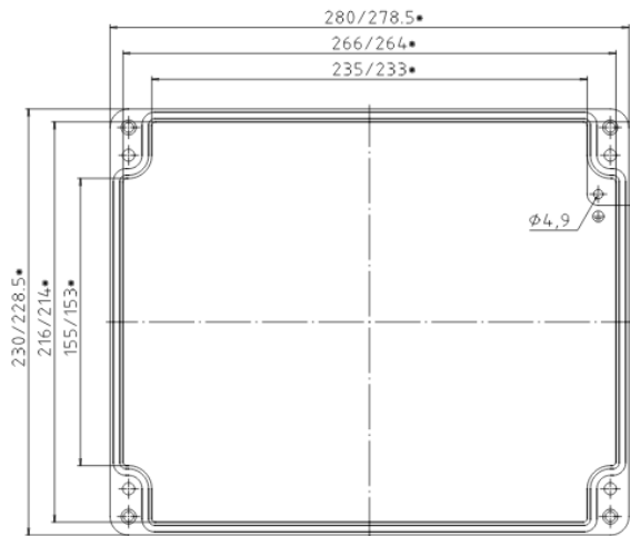
Deckel/lid
